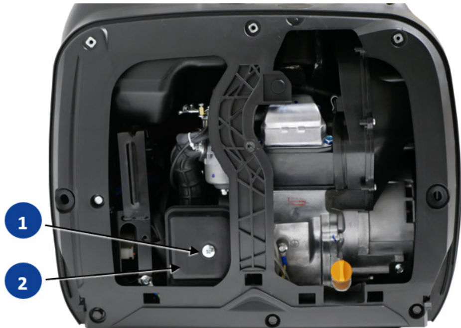
Fig. 9-3 Air filter behind the maintenance flap (removed)
