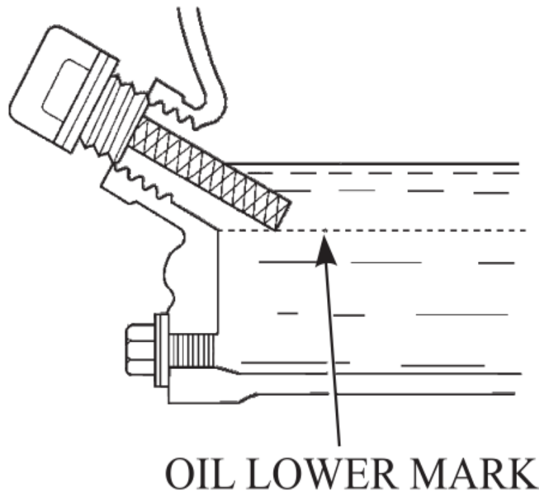
Fig. 9-2 Optimal engine oil level
