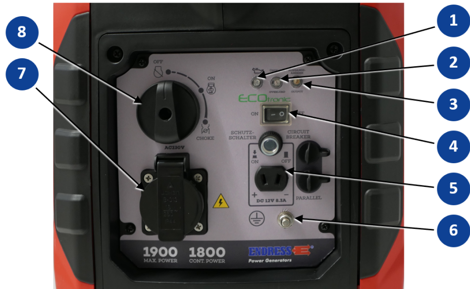
Fig. 6-4 Components on the control panel
