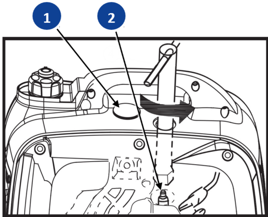
Fig. 9-4 Remove spark plug
