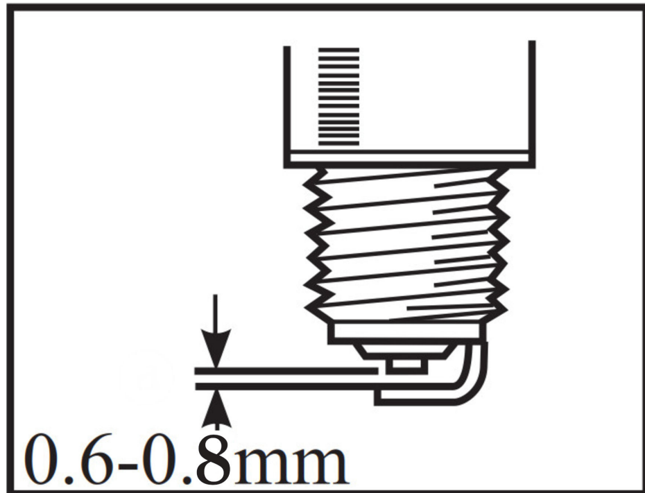
Fig. 9-5 Checking the spark plug
